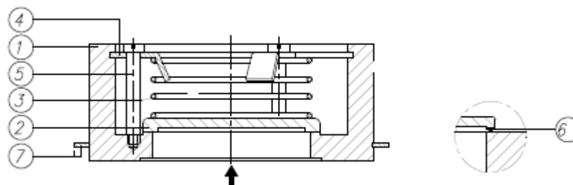
Section of wafer type check valve
